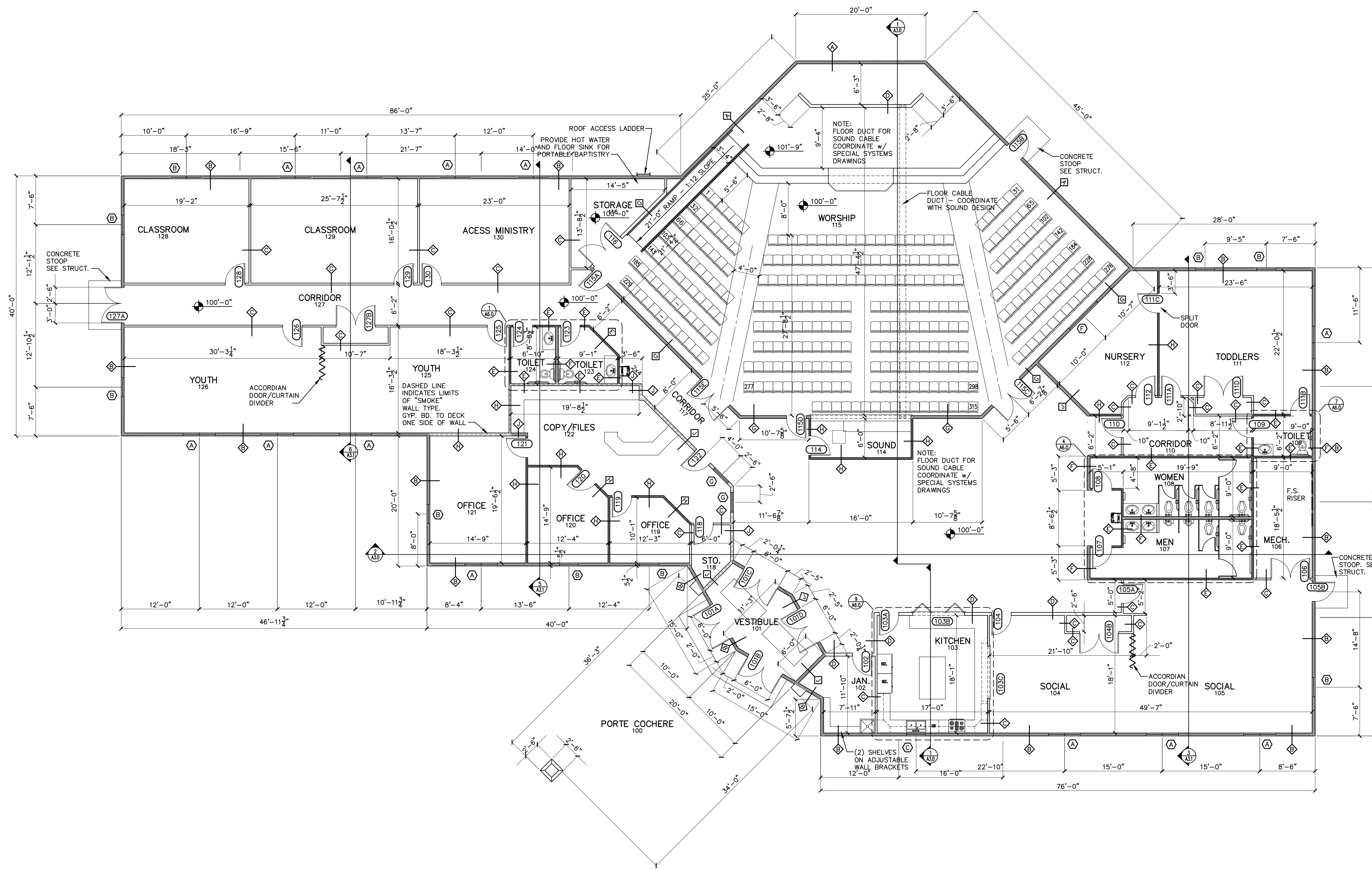
OVERALL FLOOR PLAN SCALE: 1/8" = 1'-0"
